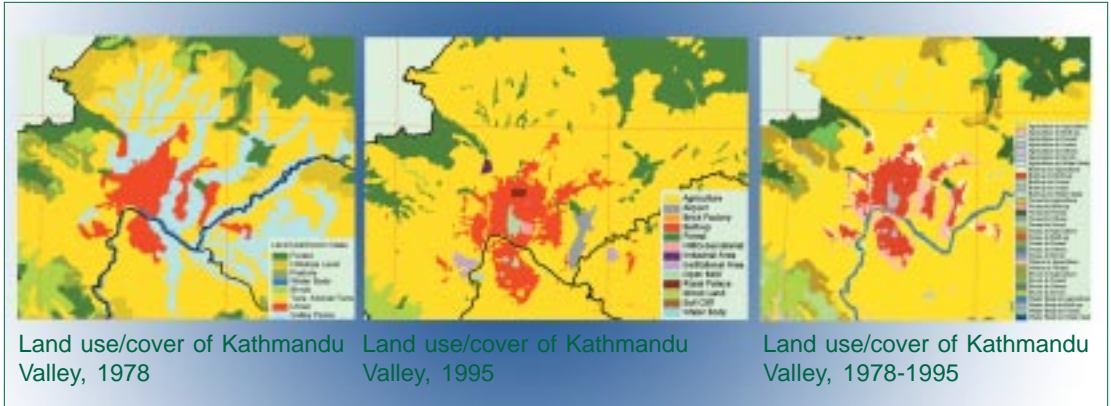
Figure 7.8
