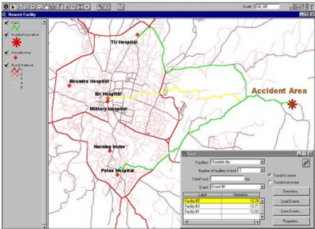
Figure 7.11 Network analysis
