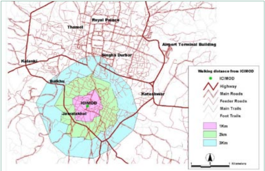
Figure 7.10
