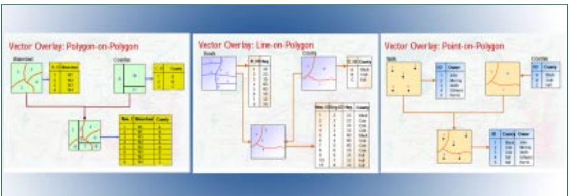
Figure 7.5 Vector overlay
