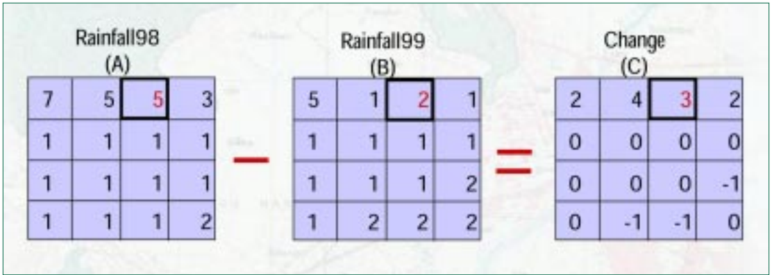
Figure 7.6 Map algebra
