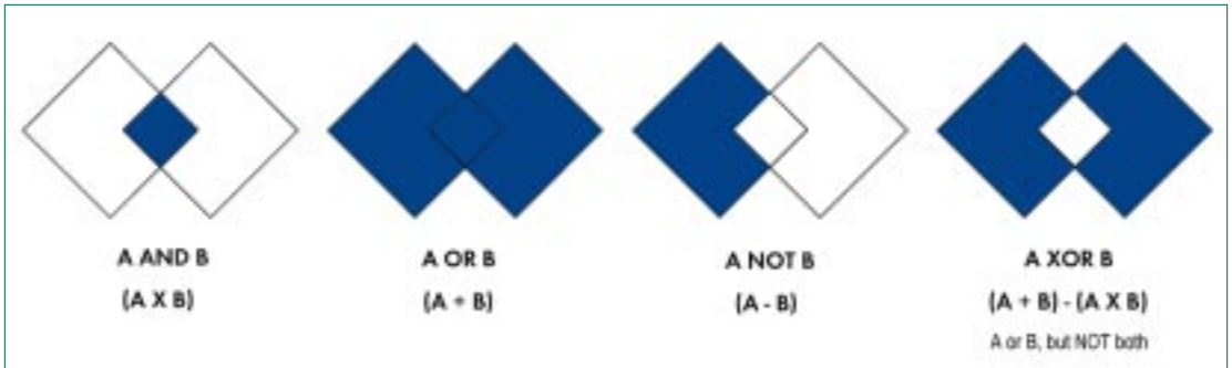
Figure 7.1 Boolean operations
