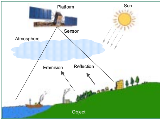
Figure 5.3 Remote-sensing
