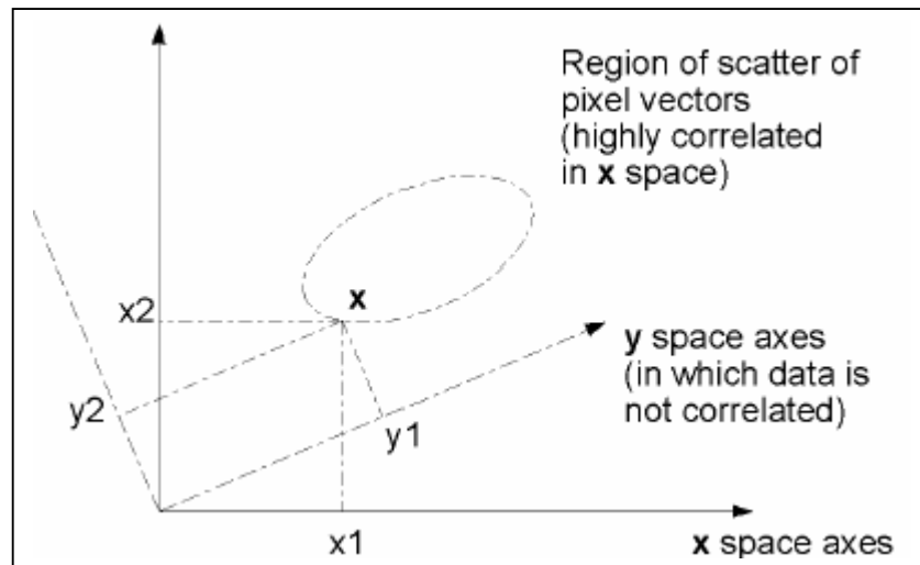
Figure 4.16 : Result of a Principal Components transformation.
