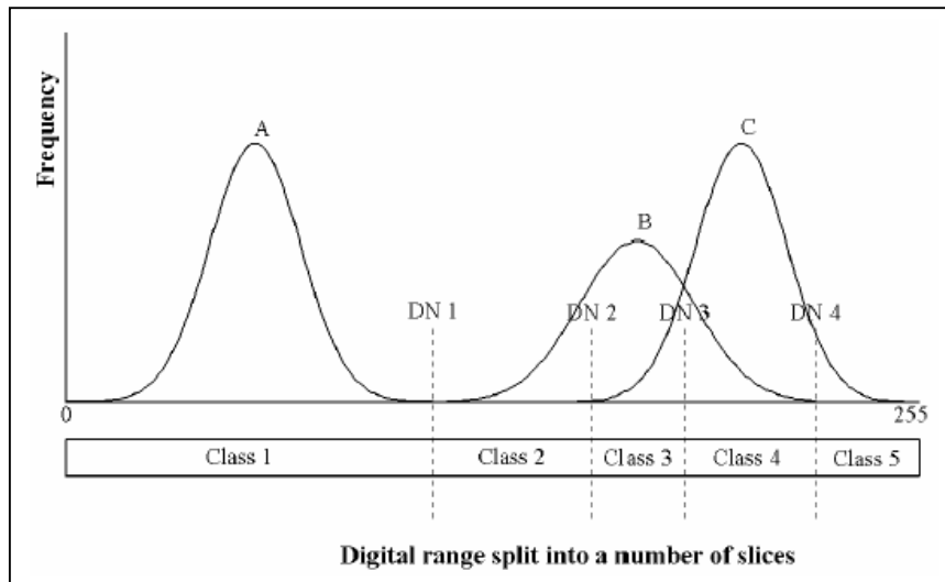
Figure 4.16: Distribution of ground cover classes over the digital range.
