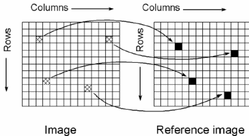
Figure 4.10: Image-to-image registration.
