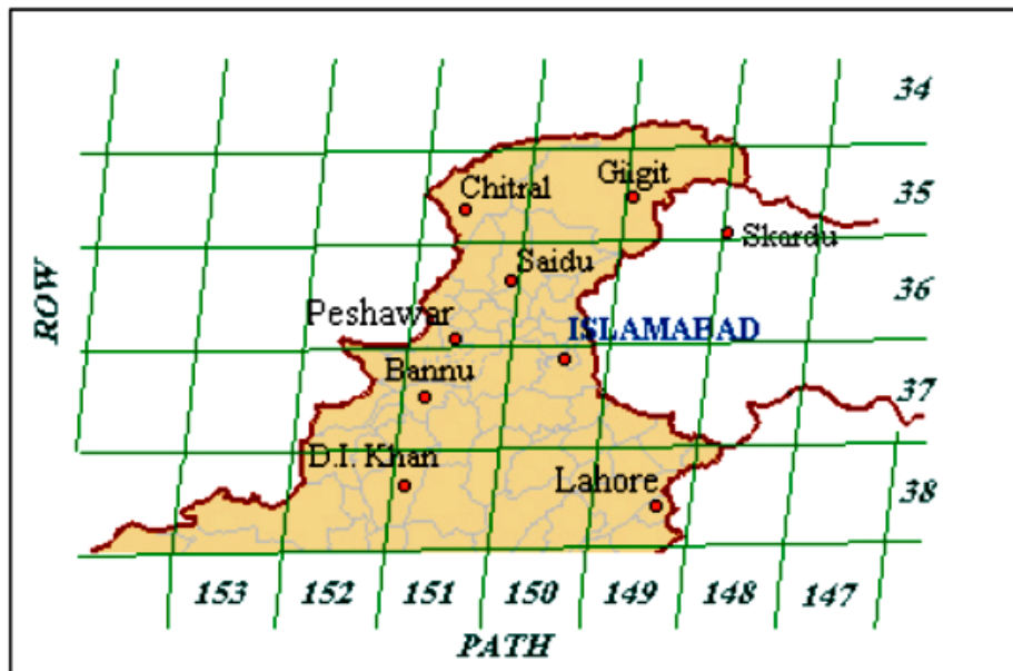
Figure: Index map of Landsat-7+ ETM scenes of Northern Pakistan.
