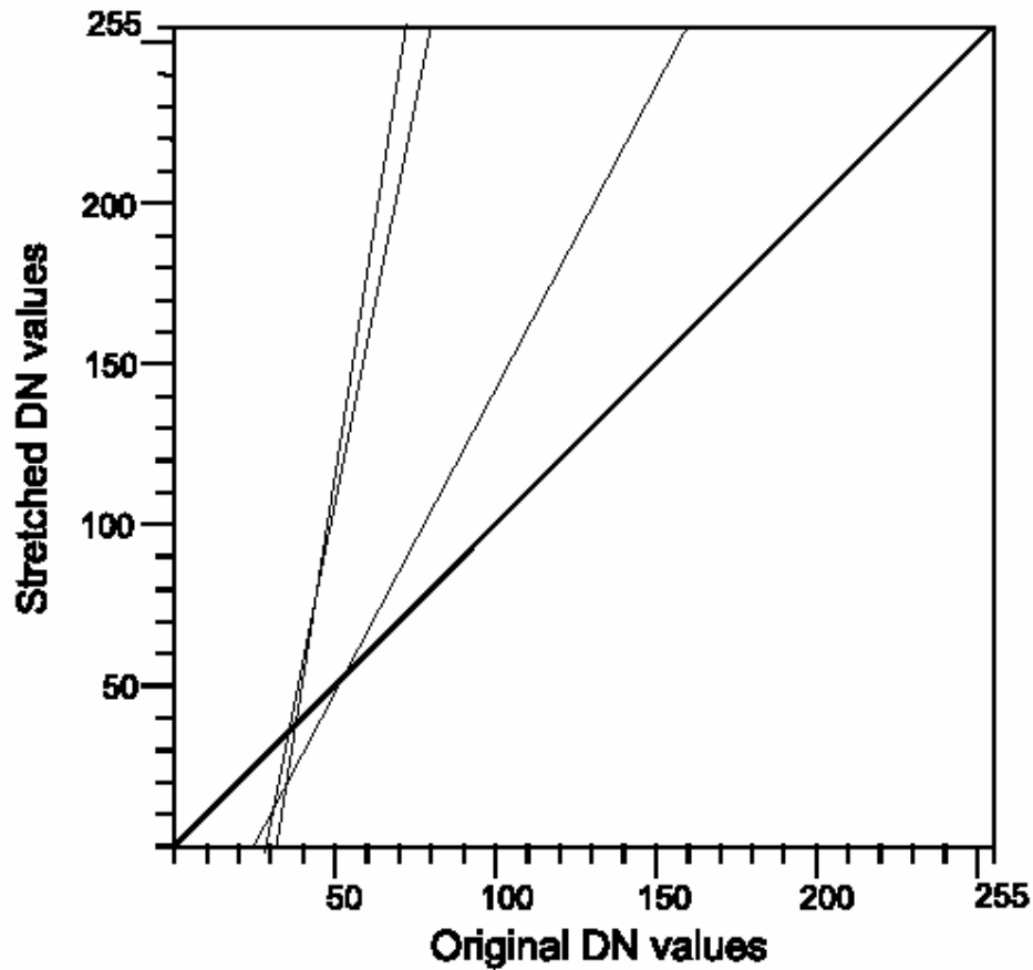
Figure 4.2: Linear stretch functions using different input intervals.
