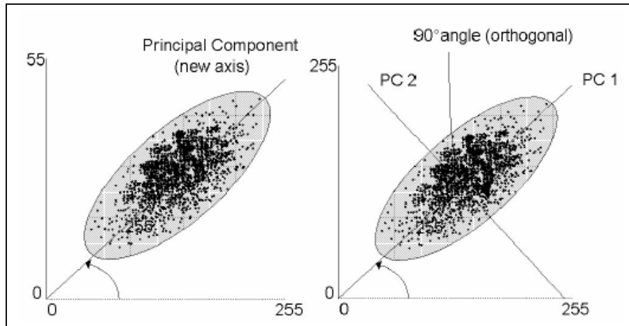
Figure 4.15: First (left) and second (right) principal components.
