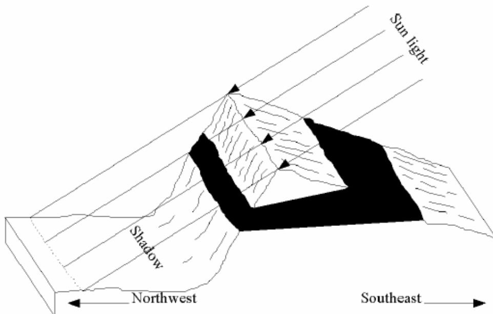
Figure 4.13: Shadow effects.
