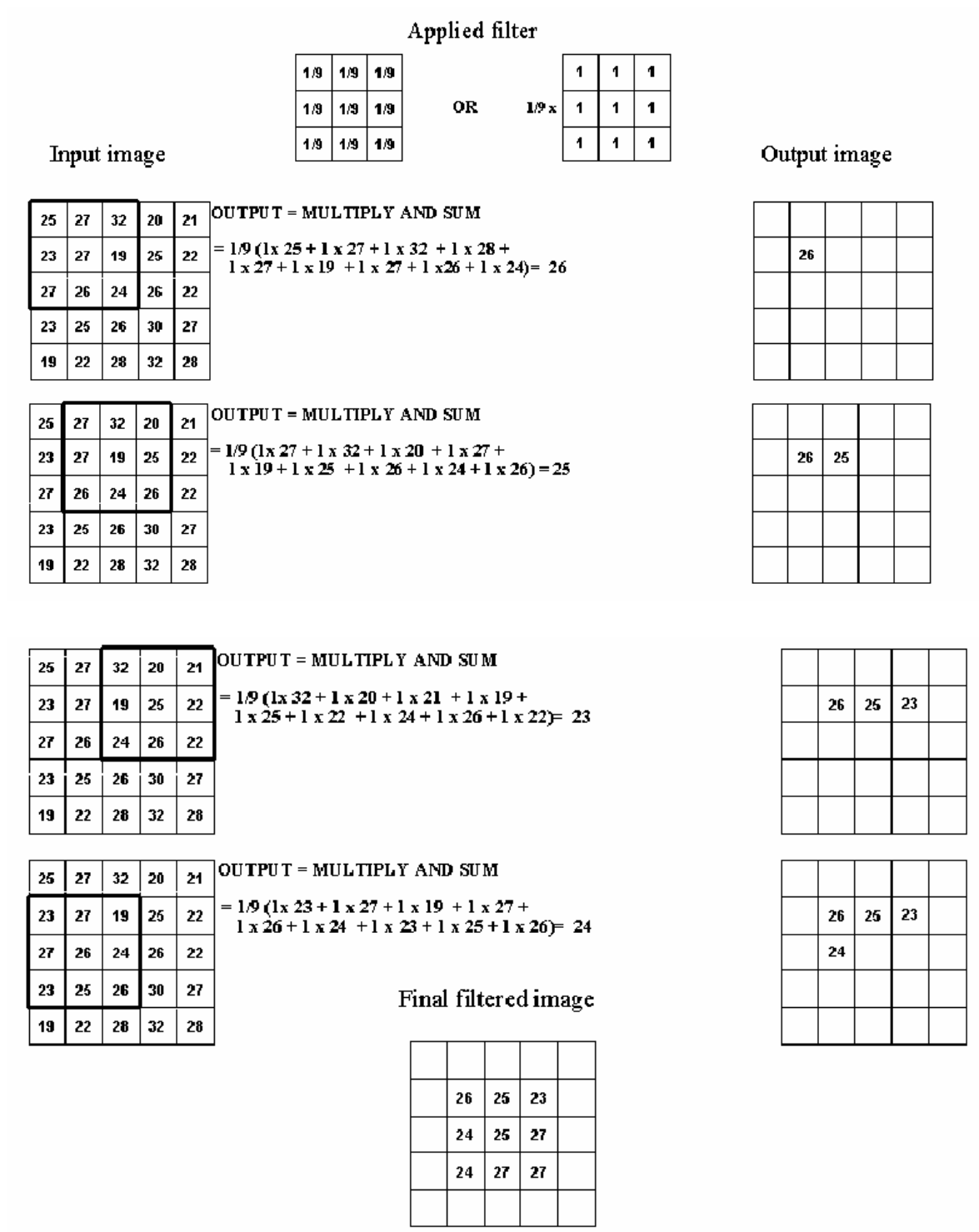
Figure 4.3 : Convolution, using a 3x3 filter with all coefficients equal to 1/9.
