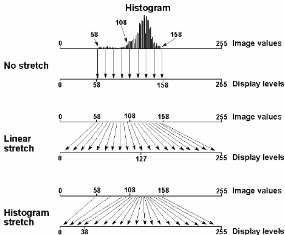
Figure 4.1 : Principle of contrast enhancement.
