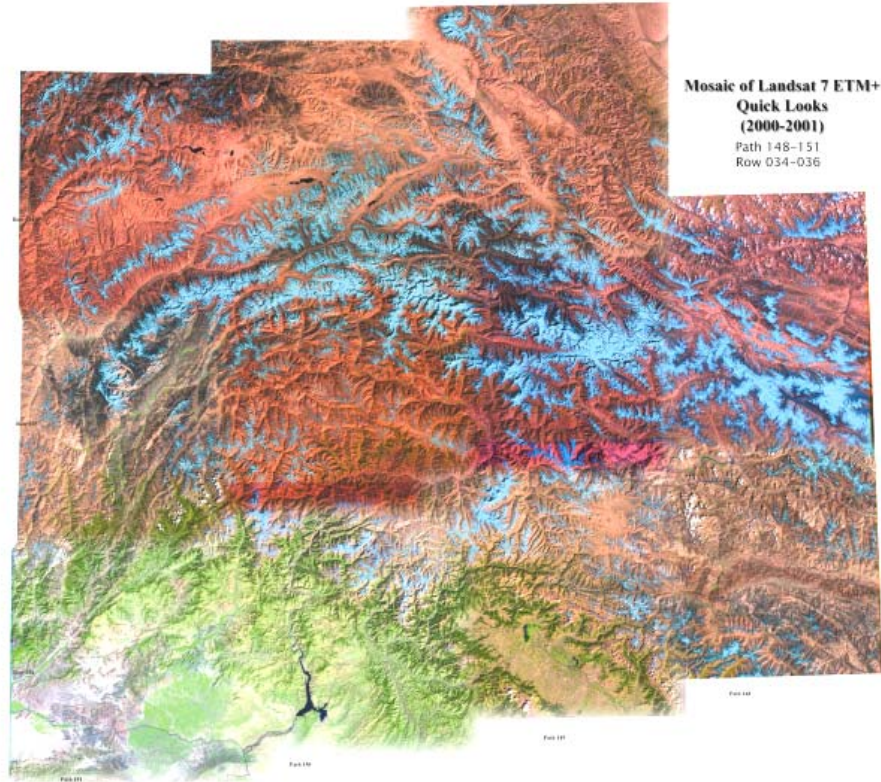
Figure: Mosaic of Landsat-7 ETM+ images of the northern Pakistan.
