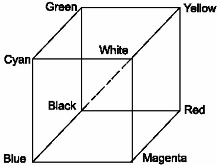
Figure 4.5 : Color cube.
