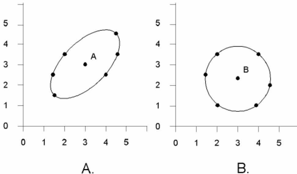
Figure 4.14 : Scatter plots showing a strong positive covariance (A) and zero covariance (B). Mean: 3.0, 3.0 (A) and 3.0, 2.3 (B).
