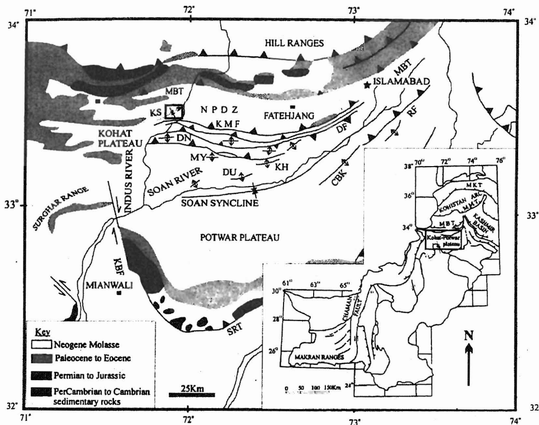
Fig. 1. Generalized map of the Kohat, Potwar and Salt Range showing prominent tectonic features (after Jaswal et al., 1997). KS (Khushalgarh syncline (after Searle and Khan, not dated). CBK= Chak Beli Khan anticline, DF=Dhurnal Fault, DJ=Dil Jabba Fault, DN=Dakhni anticline, DU=Dhulian anticline, KBF=Kalabagh Fault, KH=Khaur anticline, KMF=Kheri Murat Fault, MBT=Main Boundary Thrust, MY=Meyal anticline, RF=Riwat Fault, SRT=Salt Range Thrust
