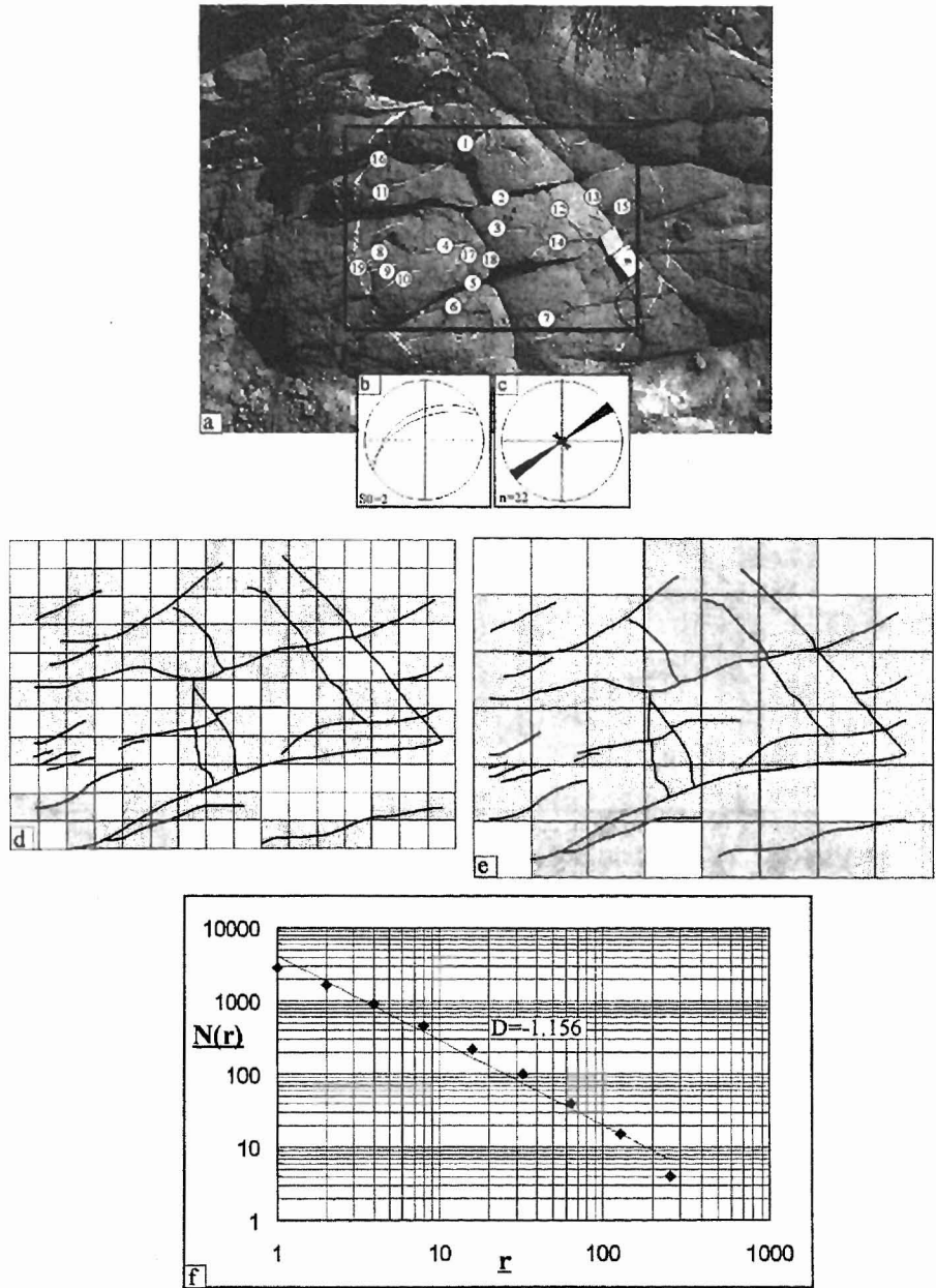
Fig. 3 (a) Fracture pattern from location A. Fractures are numbered for digitization. (b) Lower hemisphere equal area stereographic plot of S_0 . (c) Rose diagram showing fracture trends. (d and e) The box counting method for which the system is covered by a regular mesh of size r . Two different mesh sizes are shown, where boxes inside which fractures are present are shaded. (f) Standard Box counting line for fracture patterns with D=-1.156 .
