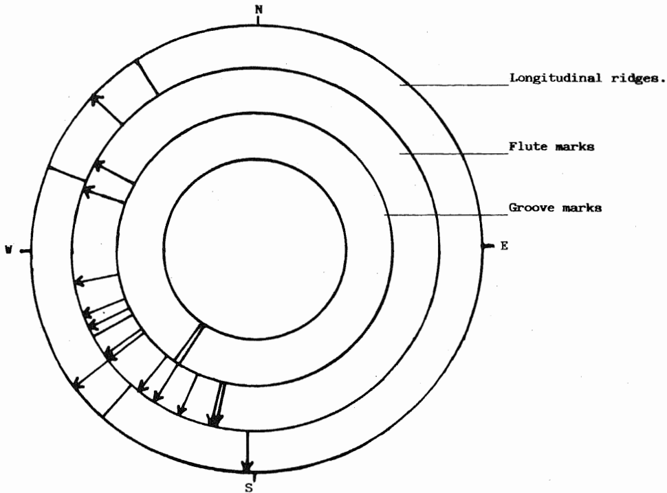
Fig. 5. Palaeocurrent directions based on sole marks (n=22).
